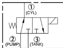
NORMALLY OPEN
