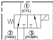
NORMALLY CLOSED
