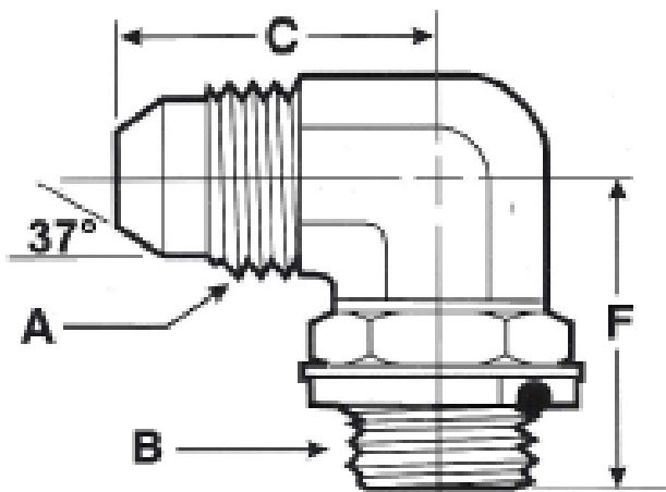
JIC Male/BSPP Male - 90° Elbow
