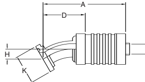
30° Elbow Split Flange FC5612 Code 61 FC5387 Code 62
