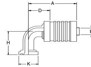
90° Elbow Split Flange
