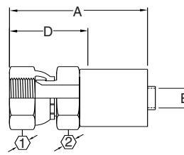
SAE 37° (JIC) swivel FC9779
